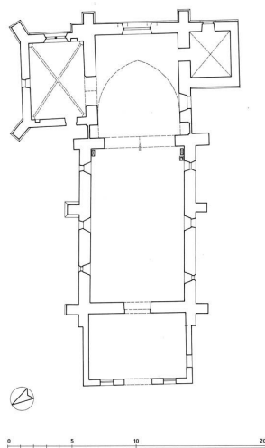
plan Dess. Alain Morelière IVR26_20122100830A2YY
