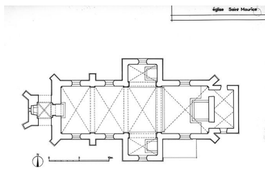
Plan au sol. Phot. Yves Sancey IVR43_19802500035V
