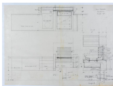
Plan du barbecue Phot. Sonia Dourlot IVR43_20167001427NUC4A
