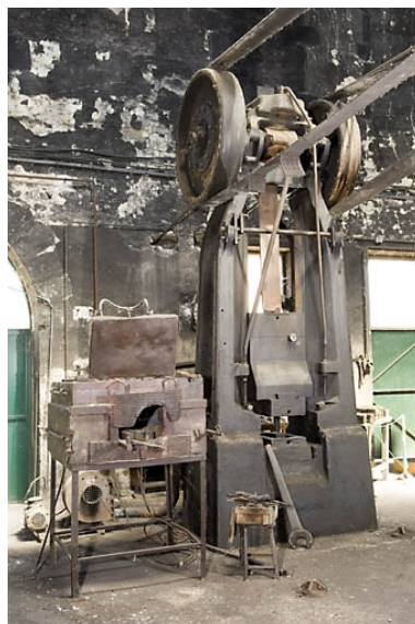
Atelier est. Marteau-pilon. Phot. Jérôme Mongreville IVR43_20087000824NUC2A
