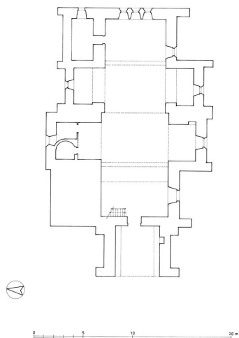
Plan. Dess. Alain Morelière IVR26_20128900011A2YY
