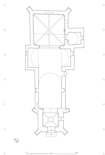
Plan. Dess. Alain Morelière, Dess. Olivier Juffard IVR26_20125800109A1YY
