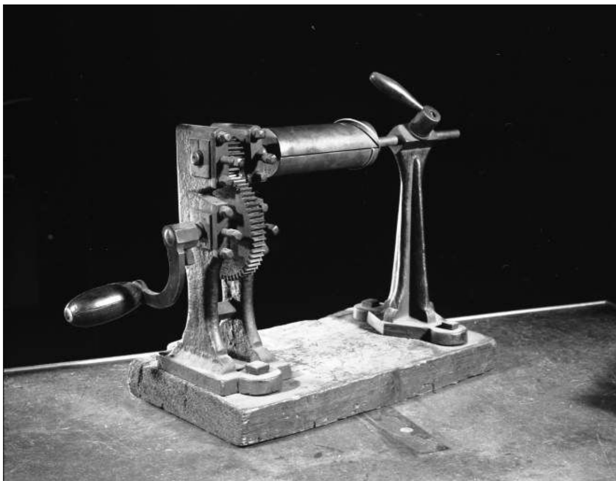
Machine à former les " cercles ".
