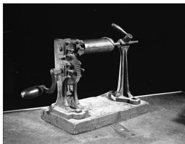
Machine à former les " cercles ". Phot. Jérôme Mongreville IVR43_19913900898X
