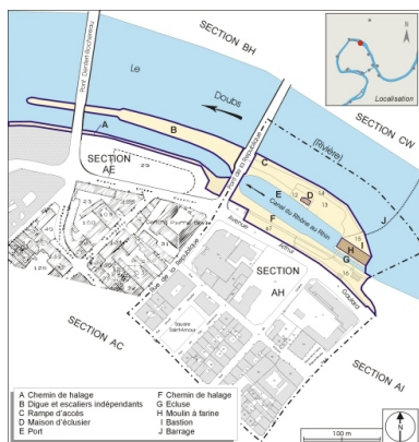
Plan-masse et de situation. Dess. André Céréza IVR43_20062500326NUDA
