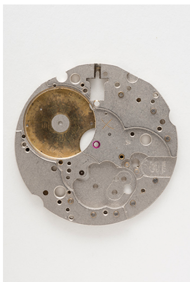
Ebauche Valjoux 7734. Phot. Sonia Dourlot IVR43_20152502558NUC4A
