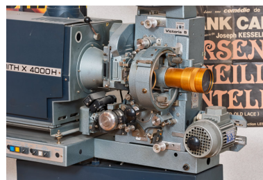
Bloc de projection. Phot. Pierre-Marie Barbe-Richaud IVR26_20245800322NUC4A
