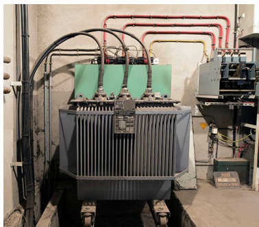
Transformateur 3 x 110 volts. Phot. Mary Ruffinoni IVR43_20147000255NUC4A
