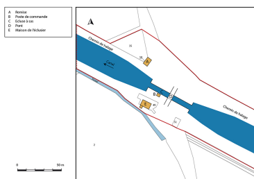
Plan masse et situation. Dess. Bertrand Turina IVR43_20207000779NUDA
