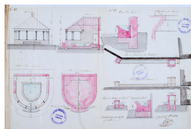
plans de la fontaine "du bas" Phot. Jérôme Mongreville, Autr. Jean-Baptiste Ridoux IVR43_20167001580NUC4A
