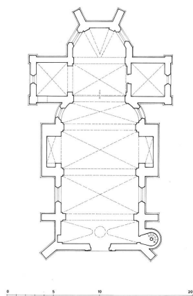
plan Dess. Alain Morelière IVR26_20122100802A2YY
