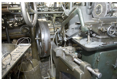
Scie horizontale alternative (G). Phot. Jérôme Mongreville IVR43_20082500052NUC2A
