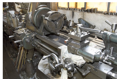
Tour horizontal parallèle Selson (A). Phot. Jérôme Mongreville IVR43_20082500049NUC2A
