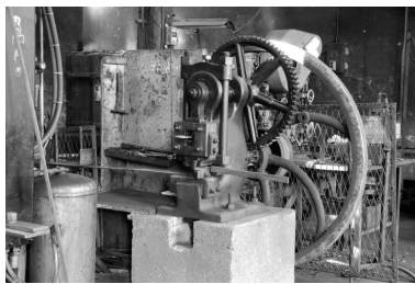
Cisaille. Phot. Laurent Poupard IVR43_19893901248Z
