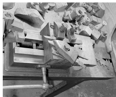
Chariot porte-outil (atelier principal). Phot. Jérôme Mongreville IVR43_20022500634X
