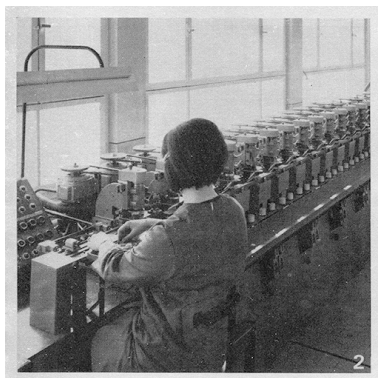
[France Ebauches] Transfert linéaire France Ebauches, 1970.
