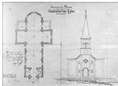
Plan, élévation principale. Phot. Yves Sancey, Phot. Achille Paillot IVR43_19833900774V
