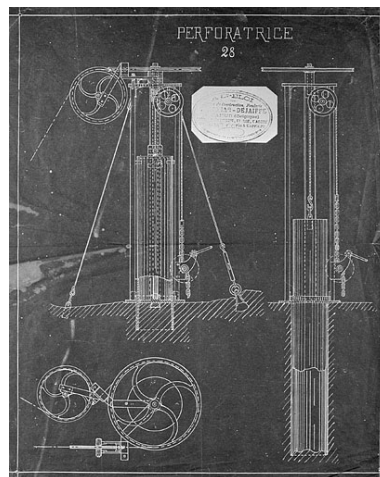
Perforatrice. Phot. Yves Sancey, Autr. Thonar Dejaiffe IVR43_19973900019X
